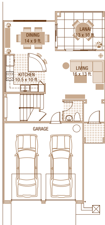
GROUND FLOOR PLAN - TYPE 2
