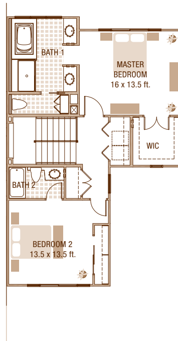
SECOND FLOOR PLAN - TYPE 2
